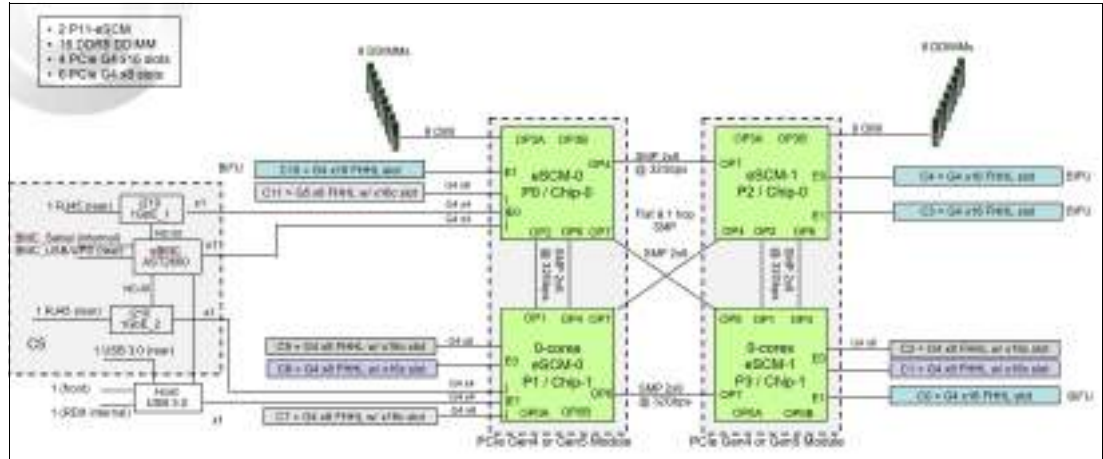
Figure 1-16 Entry Single-Chip Module logical diagram
