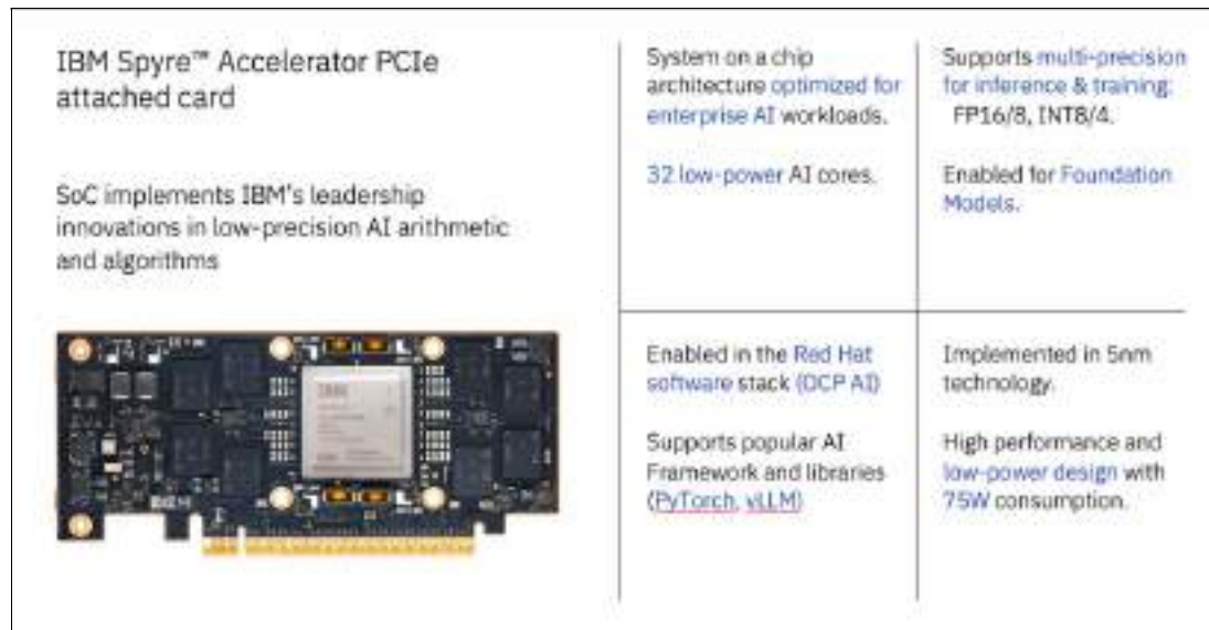
Figure 4-2 The IBM Spyre Accelerator
