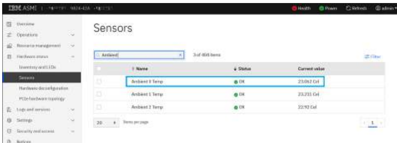
Figure 3-19 Ambient temperature readings from three sensors on the operator panel
