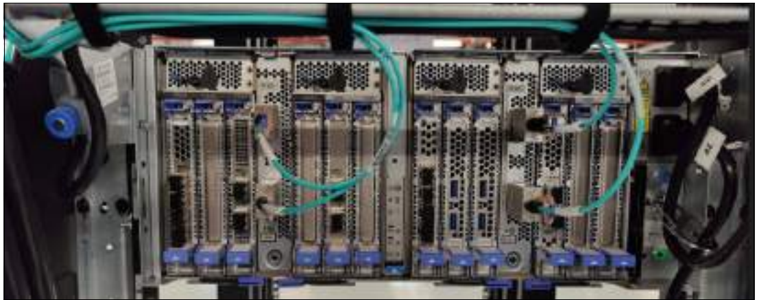
Figure 3-13 PCIe Gen 4 I/O Expansion Drawer rear view
