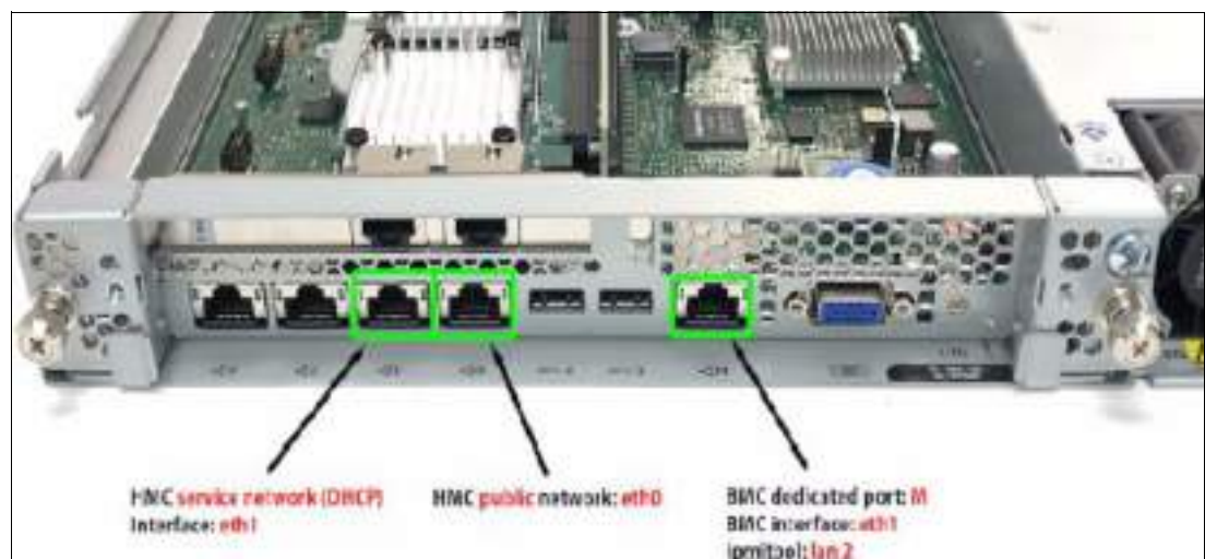
Figure 5-2 BMC interfaces
